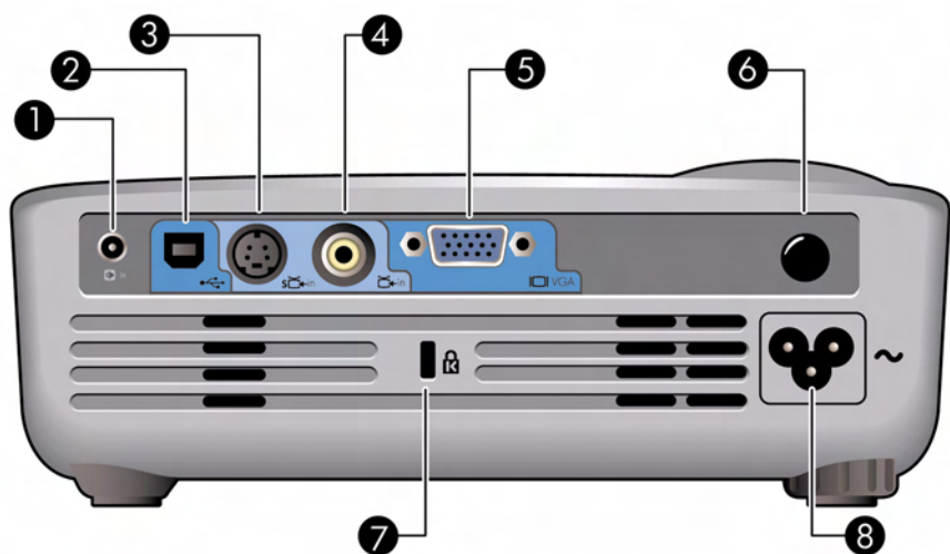
Identifying back panel components
